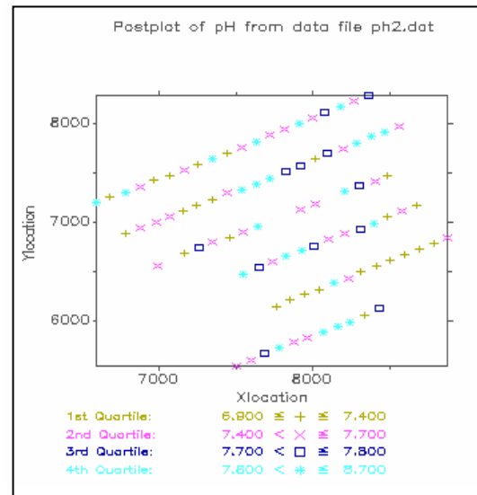
Figure 6. Post plot of soil pH quartile value
