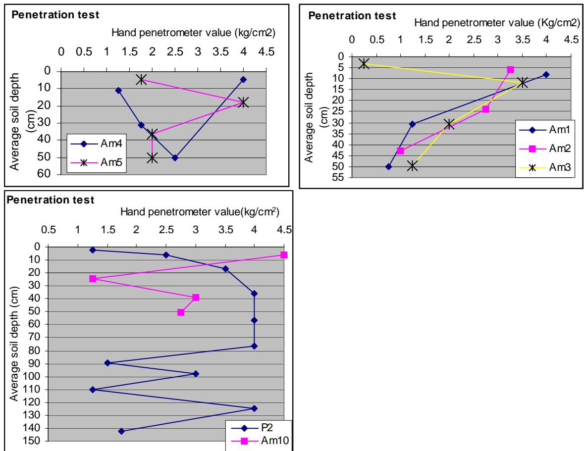
Figure 10. Penetration resistance test results using hand penetrometer for each site
