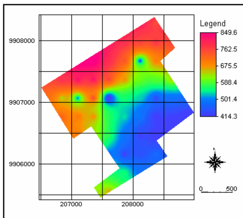
Figure 3. Topsoil EC ( \mu\text{S}/\text{cm} ) map by indicator Kriging (Longonot site, Sulmac blocks 30's-80's)
