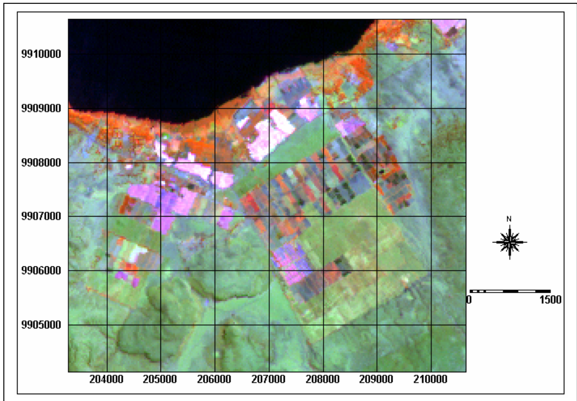
Figure 1. Satellite image of the Sulmac farm and associated areas (FCC452) form Landsat TM 2000
