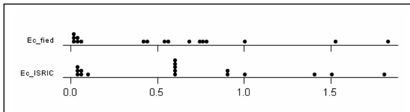
Figure 13. Dotplot between EC_field and EC_ISRIC
