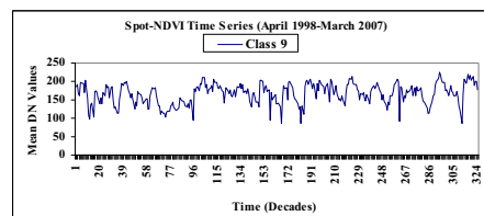
NDVI –based mapping unit one (MU1): combination of classes 6 and 9
