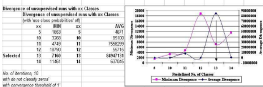
Average divergence for predefined classes with the arrow showing the classes with a peak in divergence
