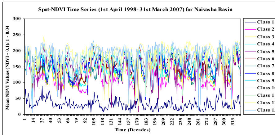
NDVI profiles of the 13 classes derived by unsupervised ISODATA clustering
