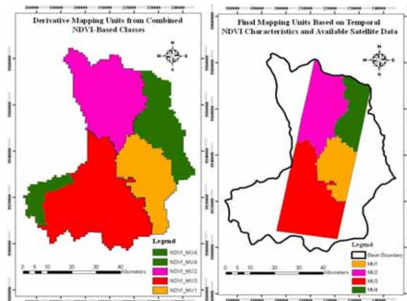
Figure 9: The mapping units delineated from the combined NDVI-based classes and, the final units based on the available satellite data
