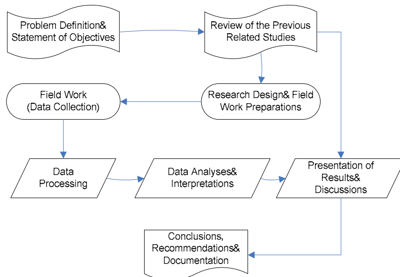
Figure 2: Flowchart illustrating the stages of the research
