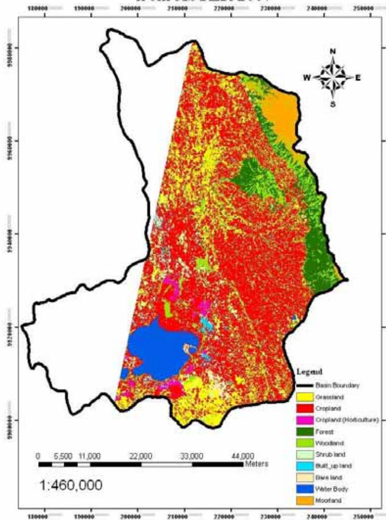
Figure 5: Land cover classification for 2007
