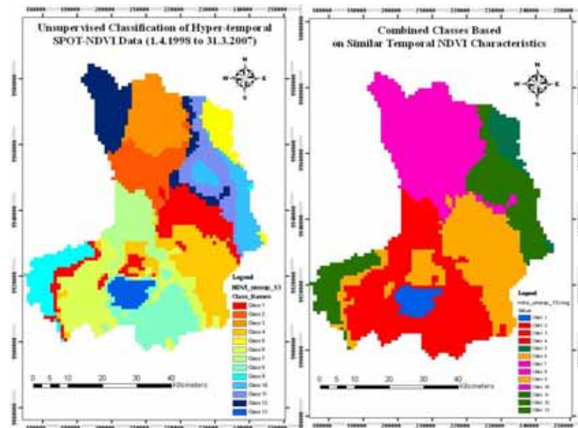
Figure 8: Unsupervised classification of SPOT-NDVI data and, the combined classes based on similar temporal NDVI behaviour
