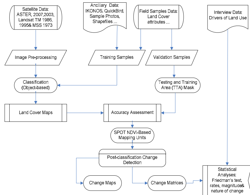
Figure 3: Schematic diagram summarizing the methods and materials
