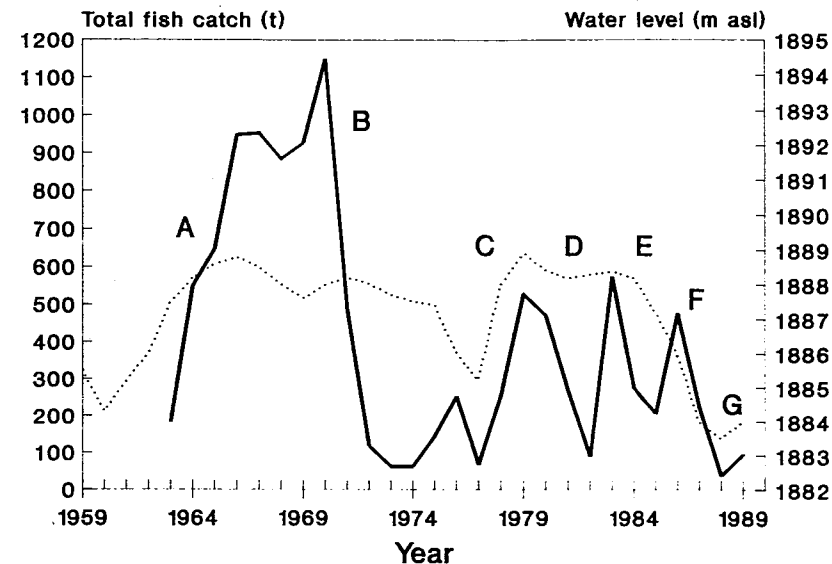
Fig. 34.2 Total catches (solid line) from the gill net fishery and water level changes (dotted line) for Lake Naivasha during the period 1963–1988 inclusive. Commercial fishing started in 1959 and records were kept from 1963. (A = period of development of the new fishery; B = period of receding lake level. Also, pressure to supply fish for processing factory led to the use of small meshed nets; C = small fishing effort (6–17 canoes) coupled with a rise in water level allowed the fishery to recover; D = period of high water but with loss of submerged plants; E = sudden decline in lake level combined with highest effort (104 canoes); F = recovery of aquatic plants but sustained high effort (49–75 canoes) and further decline in water level; G = small effort (30 canoes). Lake level starting to rise, flooding terrestrial vegetation and providing good nursery areas
