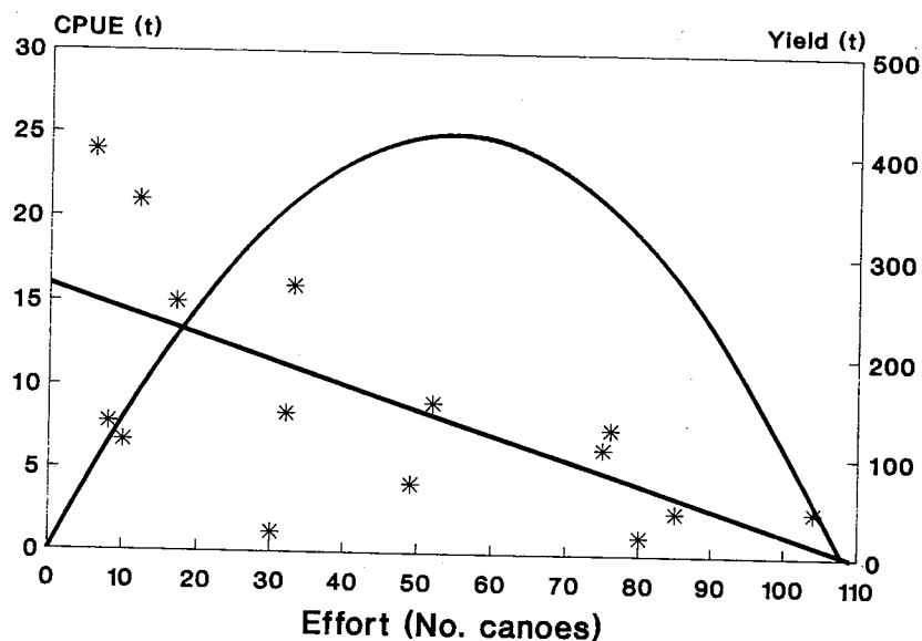
Fig. 34.1 Regression relationship (* and solid straight line) of catch per unit effort (CPUE) on effort (E) and the resulting equilibrium curve (solid curved line) for total gill net catches from Lake Naivasha for the period 1974–1988 inclusive (see also Table 34.3)
