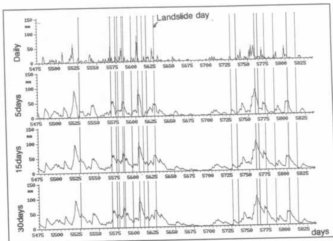
Figure 6.48: The relationship between landslide occurrences (vertical lines) and rainfall for a one year period. Daily rainfall is shown in the upper curve. Antecedent rainfall for 5, 15 and 30 days are displayed below.
