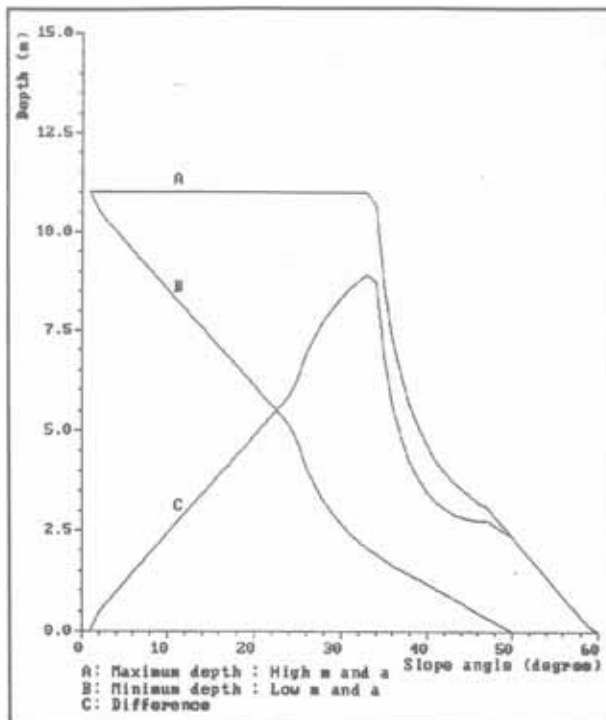
Figure 6.43: Minimum and maximum ash thicknesses based on critical depth relations.
