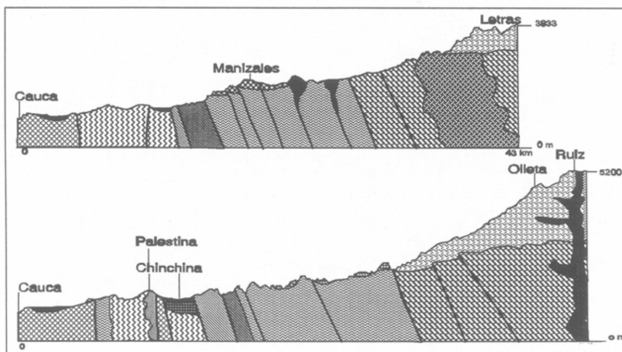
Figure 3.11: Generalized geological profile through the study area from west to east. The location of the profile is indicated in figure 3.2. The legend is shown in table 3.4.
