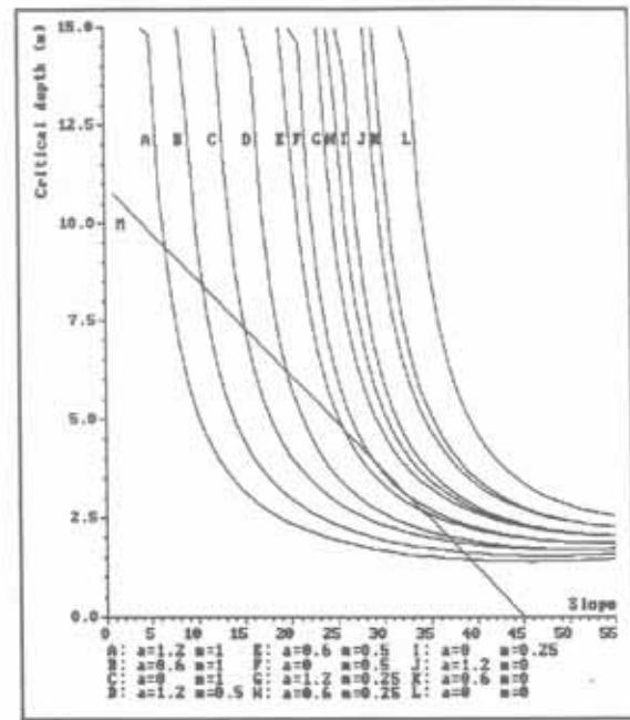
Figure 6.37: Critical depth plotted against surface slope angle for various combinations of values for seismic acceleration ( a ) and groundwater ( m = z_w/z ). Line M displays the relationship between ash thickness and slope angle used in this study.
