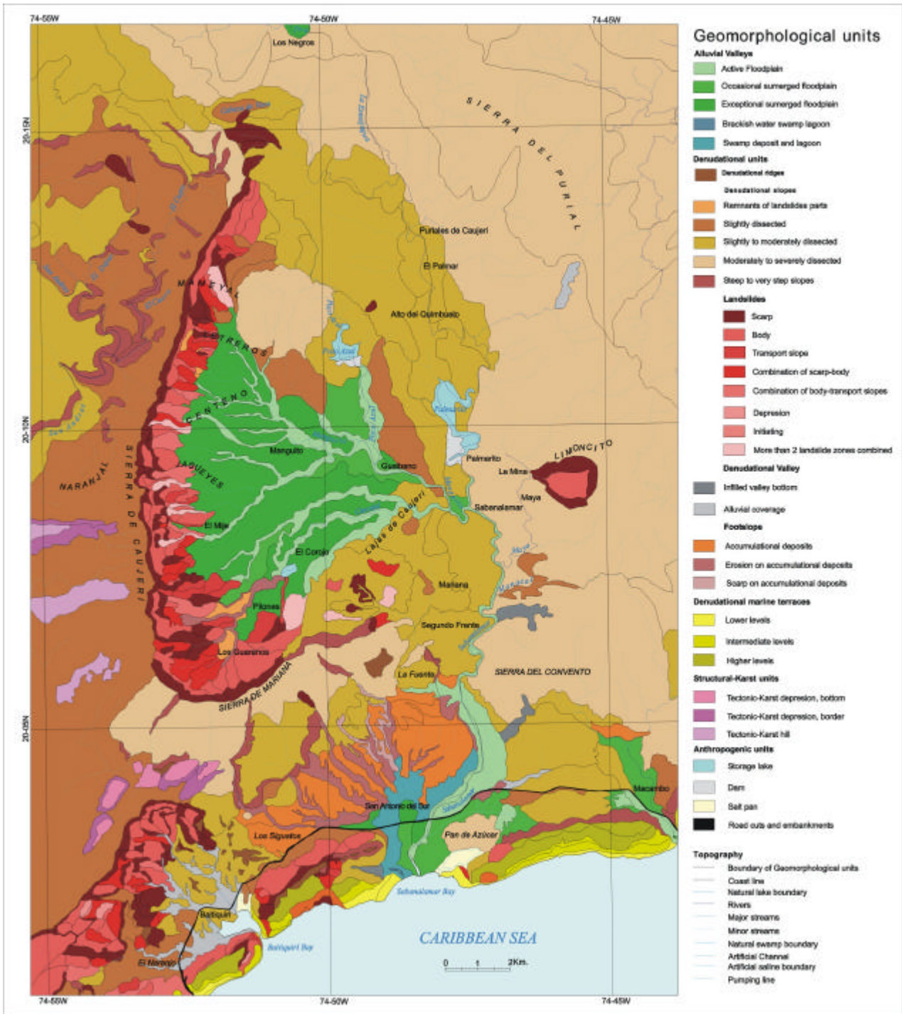
Figure 2: Geomorphological map. San Antonio del Sur, Guantánamo Province, Cuba.
