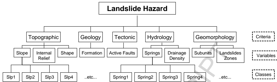
Figure 5: Components of the heuristic landslide hazard model.
