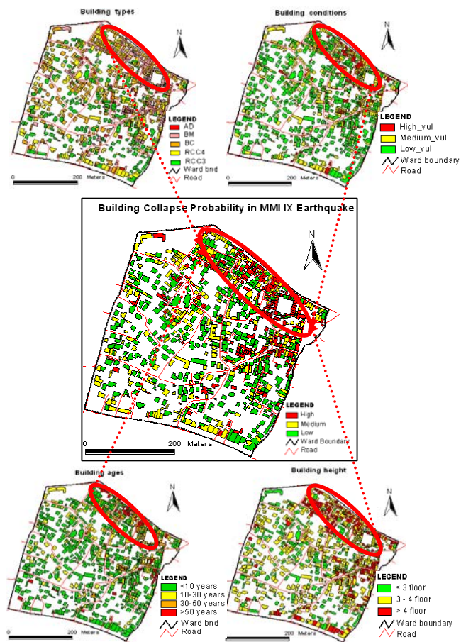
Figure 1: Building Collapse Probability in Scenario Earthquake
