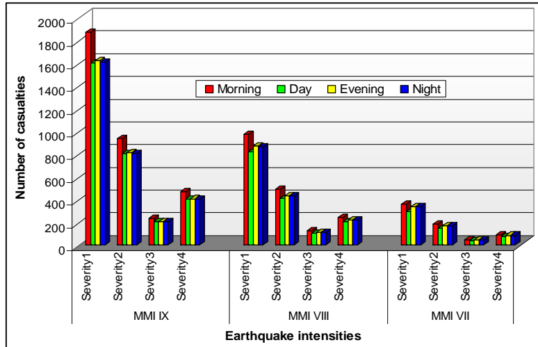
Figure 3: Casualties due to different earthquake intensities
