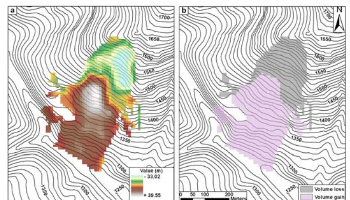
Figure 2 Volumetric analysis of the Salna landslide based on satellite derived DTMs. (a) elevation difference due to the landslide with negative values showing lowering of surface and positive values showing rising of the surface after the event, and (b) extent of the volume loss and volume gain, which corresponds to the zones of depletion and accumulation, respectively (Martha et al., 2010b).
