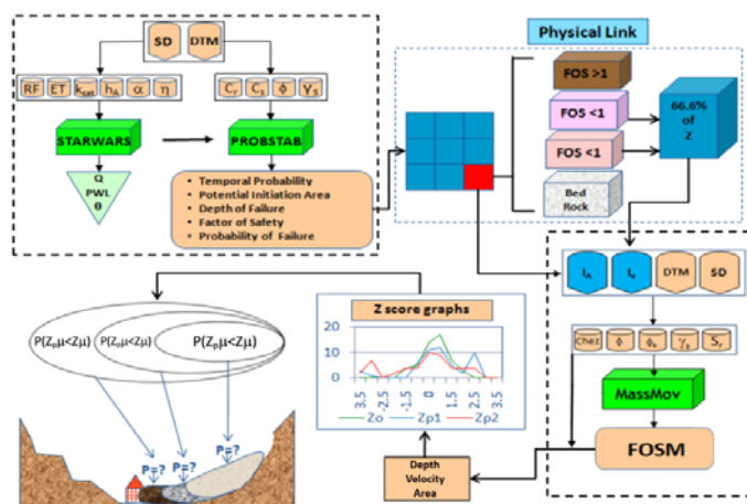
Figure 9 Scheme for coupling the results of STARWARS+PROBSTAB with the runout model MassMov2D.
