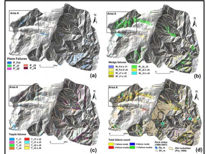
Figure 6 Modelled unstable slopes for different types of rock slope failure (a) plane failure (b) wedge failure (c) topple failure (d) slopes where at least one failure mode is kinematically possible.
