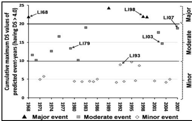
Figure 5 Threshold cumulative discriminant scores (DS) for predicted “minor”, “moderate” and “major” landslide events. The available six events are shown and associated with corresponding inventory numbers to depict validity of model-derived severity classifications of known landslide events.
