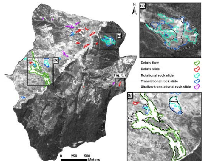
Figure 4 Landslide types recognised using OOA in the Okhimath area. The dotted lines in insets (b) and (c) show the reference landslide inventory (Martha et al., 2011a)
