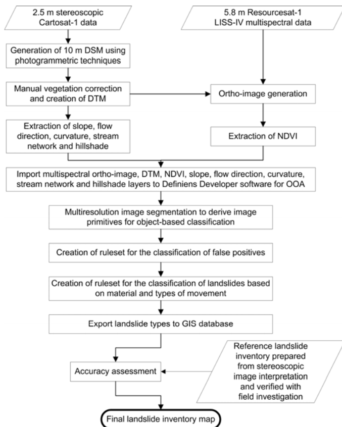
Figure 3 Generalised methodology flowchart for semi-automatic detection of landslides using object-based methods (Martha et al., 2010c).
