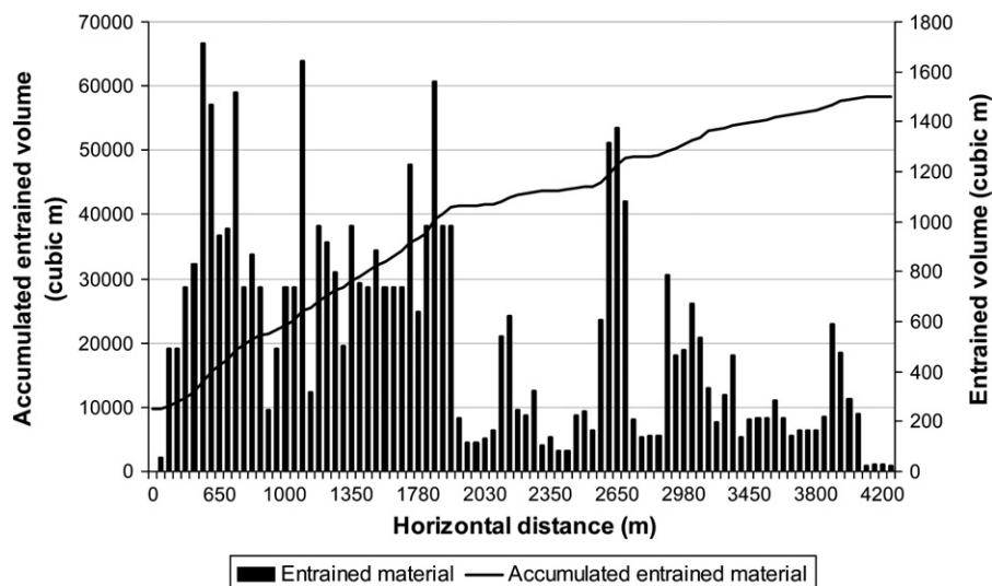
Fig. 10. Cumulative volumes of the deposits during the entrainment process and the entrained volume during the course of the flow.
