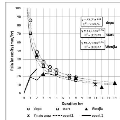
Figure 5: Graphs showing calculated combinations of critical rain intensity ( mm\ hr^{-1} ) and duration for the start ("Shuida start") and critical run-out ("Shuida depo") of debris flows in the Shuida catchment. The graphs are compared with a threshold graph for the triggering of debris flows in the Wenjia catchment which is constructed on the basis of 5 triggering rain events with different mean intensity and duration.
