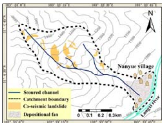
Figure 2 Geomorphological map of the Shuida catchment with co-seismic landslides and a depositional fan caused by the August 2011 debris flows
