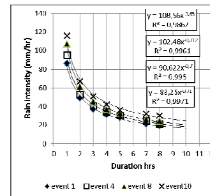
Figure 6: Changes in the threshold graphs after respectively 1, 4, 8, and 10 consecutive rain events with a certain intensity and duration.
