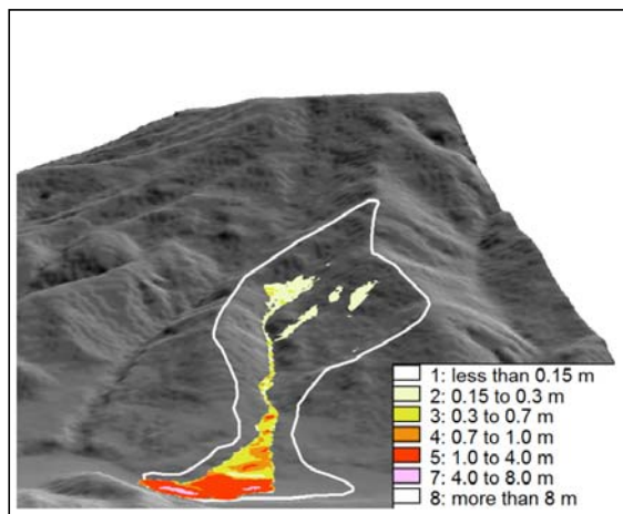
Figure 4 Simulated debris flow deposits in the Shuida catchment after the August 13 and 18 debris flow events. The white line in the flood plane is the observed limit of spreading of the debris flow materials. (See also Fig 2.) This spreading could not be simulated quite well due to the limited resolution of the DEM
